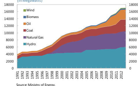
Installed Capacity by Source (In Megawatts)
