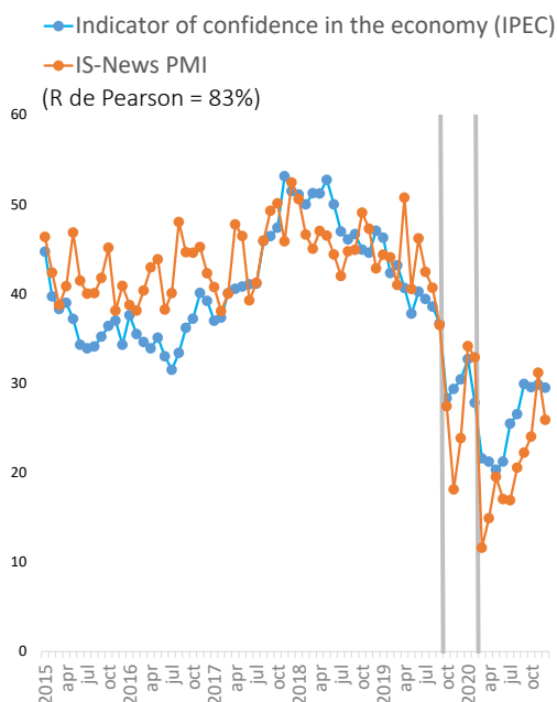
Figure 2: IS-News vs Indicators of Confidence in the Economy (IPEC): 2015-2020
