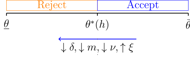
Figure 4: Threshold \theta^*(h) as a function of model parameters.
