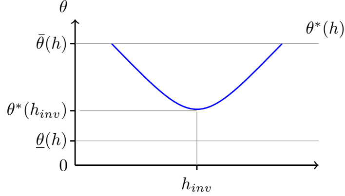
Figure 5: Threshold \theta^*(h) as a function of the haircut.
