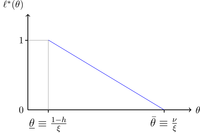
Figure 3: Threshold \ell^*(\theta) .
