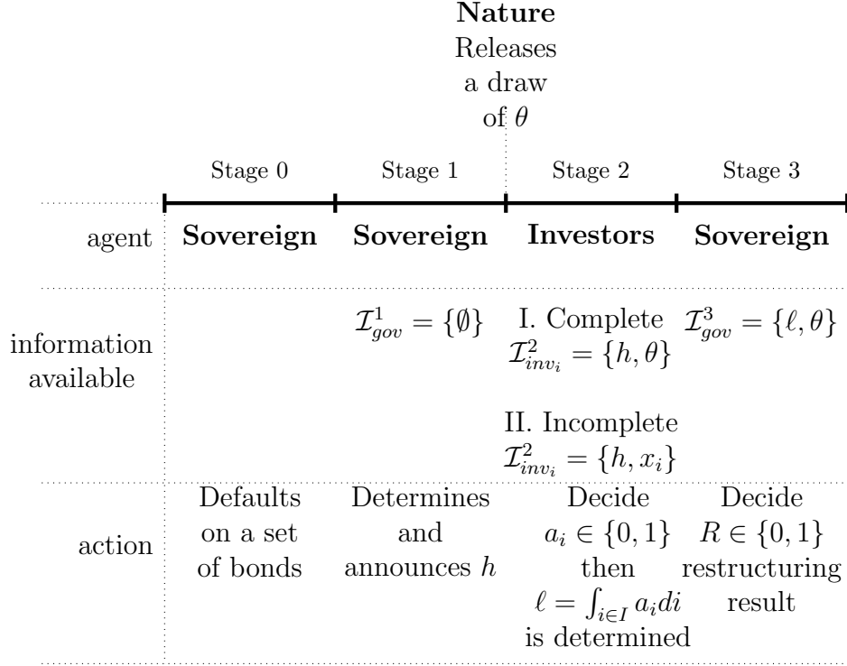
Figure 2: Model Structure and Timeline.
