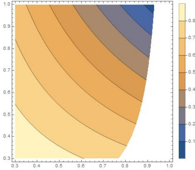
Figure 6: Simulated haircut as a function of model parameters. Contour plot: h_{co} as a function of \delta (abscissa) and \nu (ordinate), with m = 0.013 , \xi = 0.04 and an exponential distribution of \theta with \lambda = 0.16 . The white region does not satisfy the conditions in Lemma 3.
