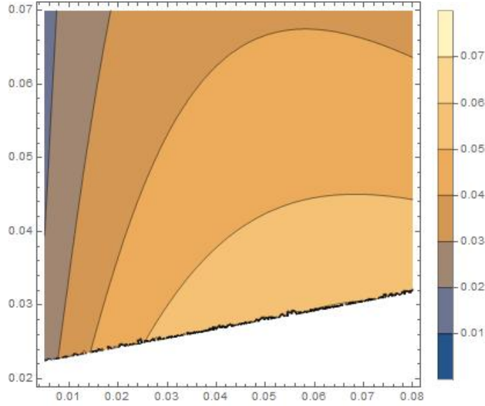
Figure 9: Coordination costs against model parameters. Contour plot: coordination costs as a function of m (abscissa) and \xi (ordinate), with \delta = 0.375 , \nu = 0.835 , assuming an exponential distribution of \theta with parameter \lambda = 0.16 . The white zone does not satisfy Lemma 3.
