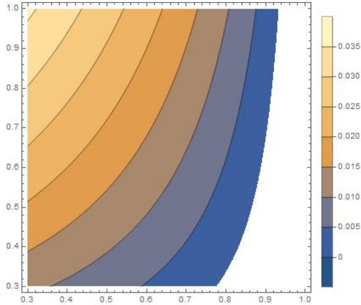
Figure 8: Coordination costs against model parameters. Contour plot: coordination costs as a function of \delta (abscissa) and \nu (ordinate), with m = 0.01 , \xi = 0.04 , assuming an exponential distribution of \theta with parameter \lambda = 0.16 . The white zone does not satisfy Lemma 3.
