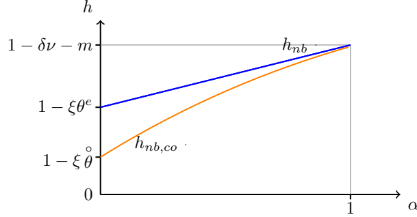
Figure 10: Nash and coordination haircut.
