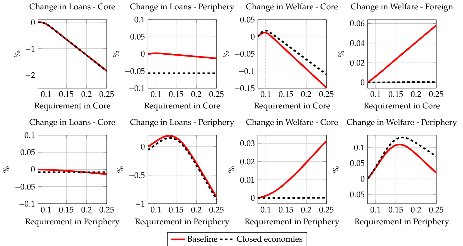
Figure A.5: Long run effects in the asymmetric setting
