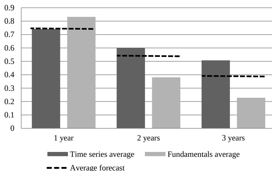
Figure 11: RMSE of average models (relative to RMSE of Mod.1)
