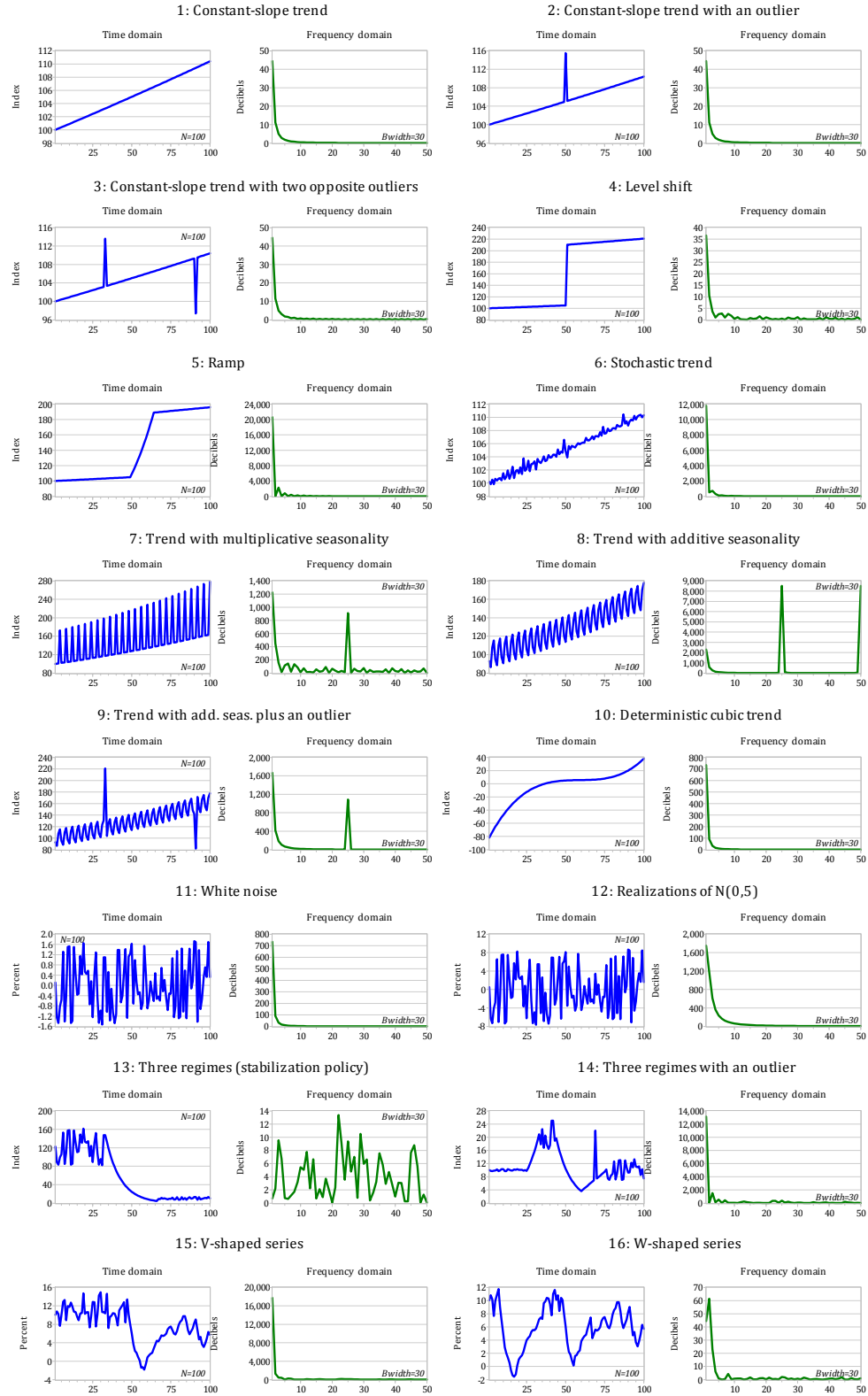
Figure 2: Basic estimations
