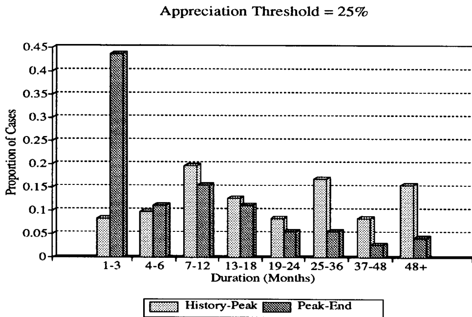
Figure 23: Phases Duration - Trends Only
