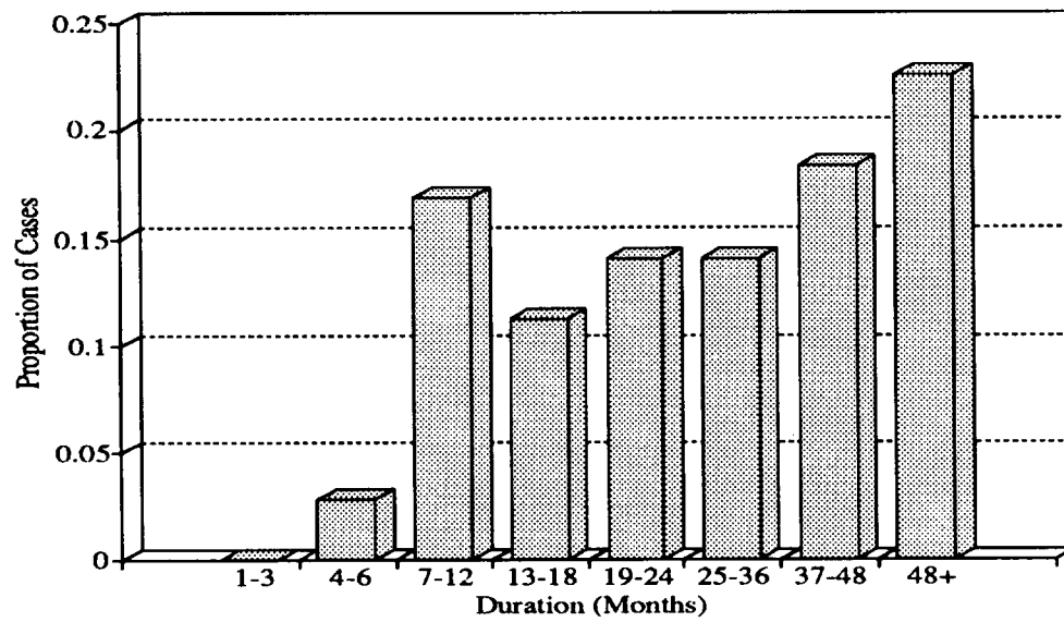
Figure 21: Histogram of Duration - Trends Only
