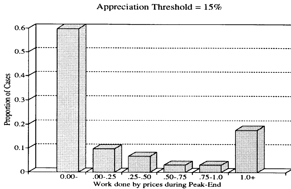
Figure 9: Histogram of Smoothness - Trends Only (15%)
