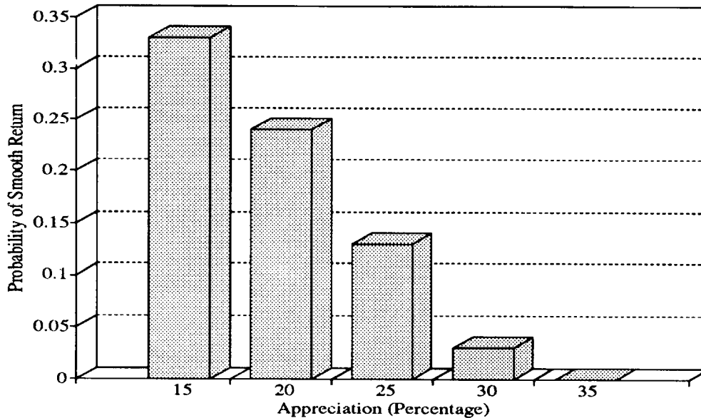
Figure 1: Probability of Smooth Return Appreciation
