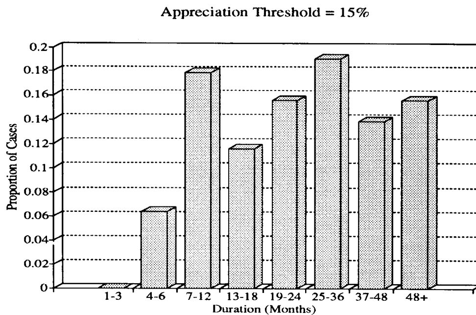
Figure 3: Histogram of Duration - Trends Only
