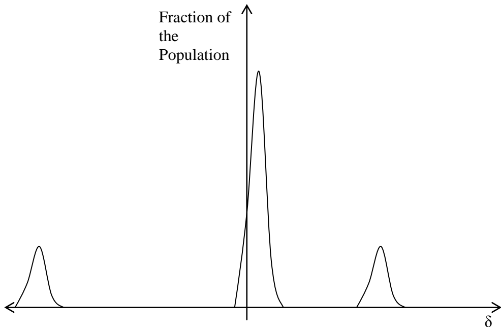
Example of a Distribution of \delta s in the Population
